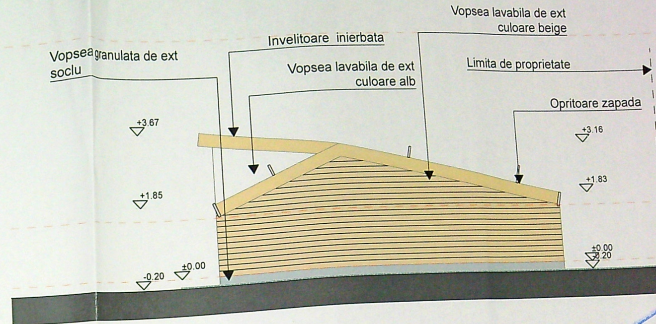
Fatada Vest
