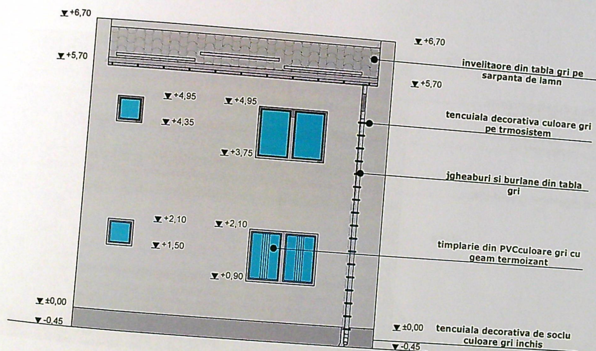
FATADA VEST SCARA1:100
