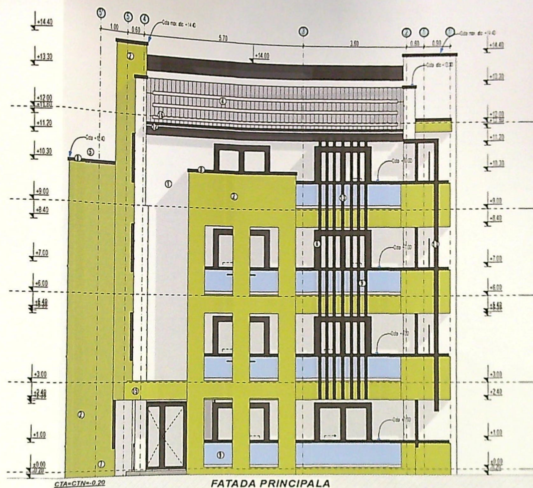
FATADA PRINCIPALA
