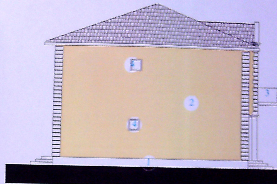
FATADA VEST
