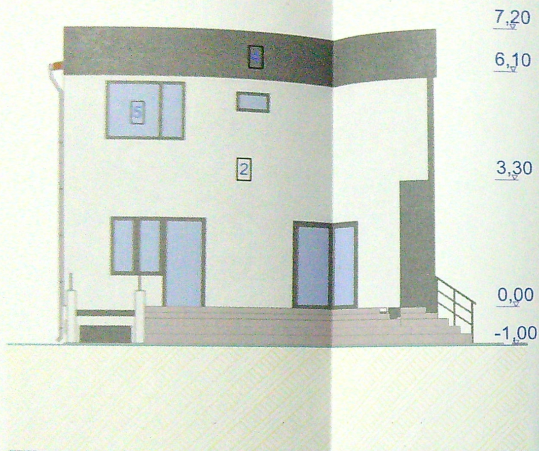
FATADA STANGA scara 1:100
