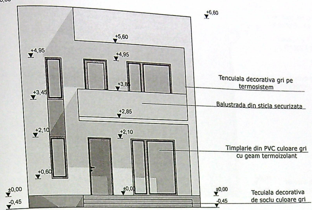
FATADA VEST SCARA1:100
