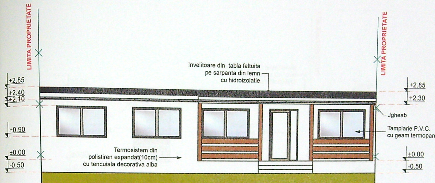
FATADA PRINCIPALA Scara 1:100
