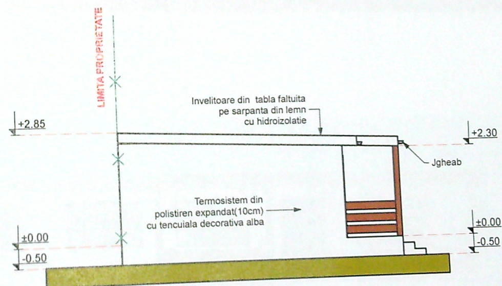
FATADA LATERALA STANGA Scara 1:100
