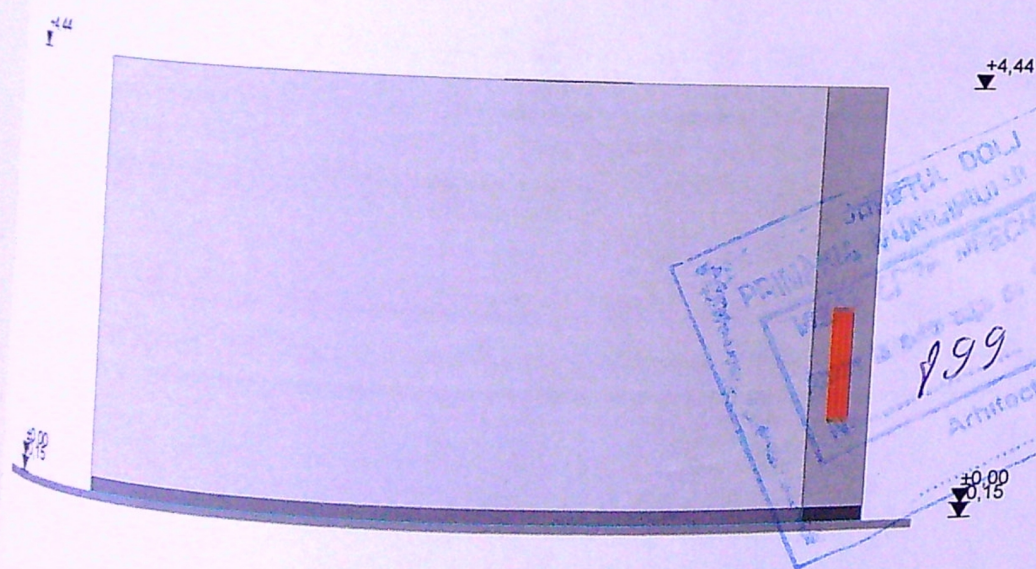
FATADA VEST SCARA1:100
