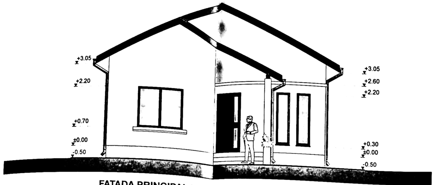
FATADA PRINCIPALA
