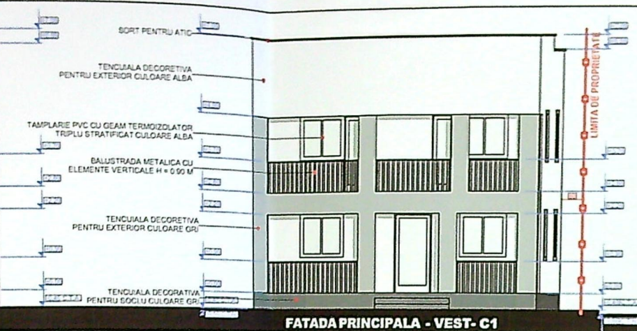
FATADA PRINCIPALA - VEST- C1
