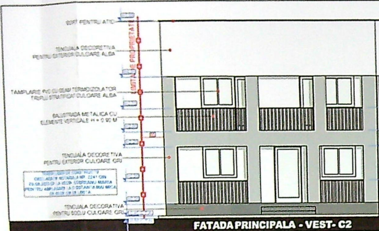
FATADA PRINCIPALA - VEST- C2
