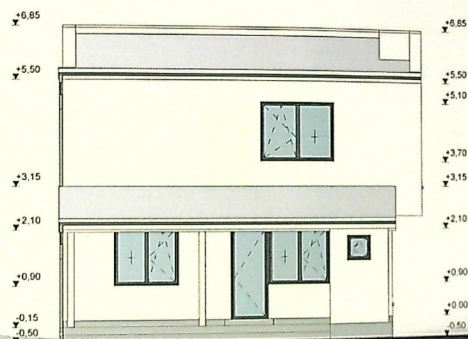
FATADA PRINCIPALA
