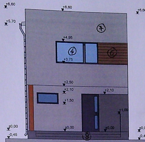
FATADA VEST SCARA1:100
