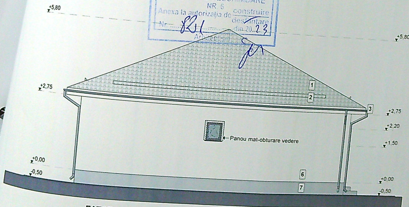
FATADA LATERALA STANGA (FATADA NORD)
