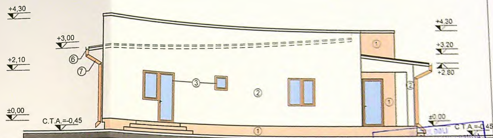
FATADA LATERALA STANGA (NORD - EST)
