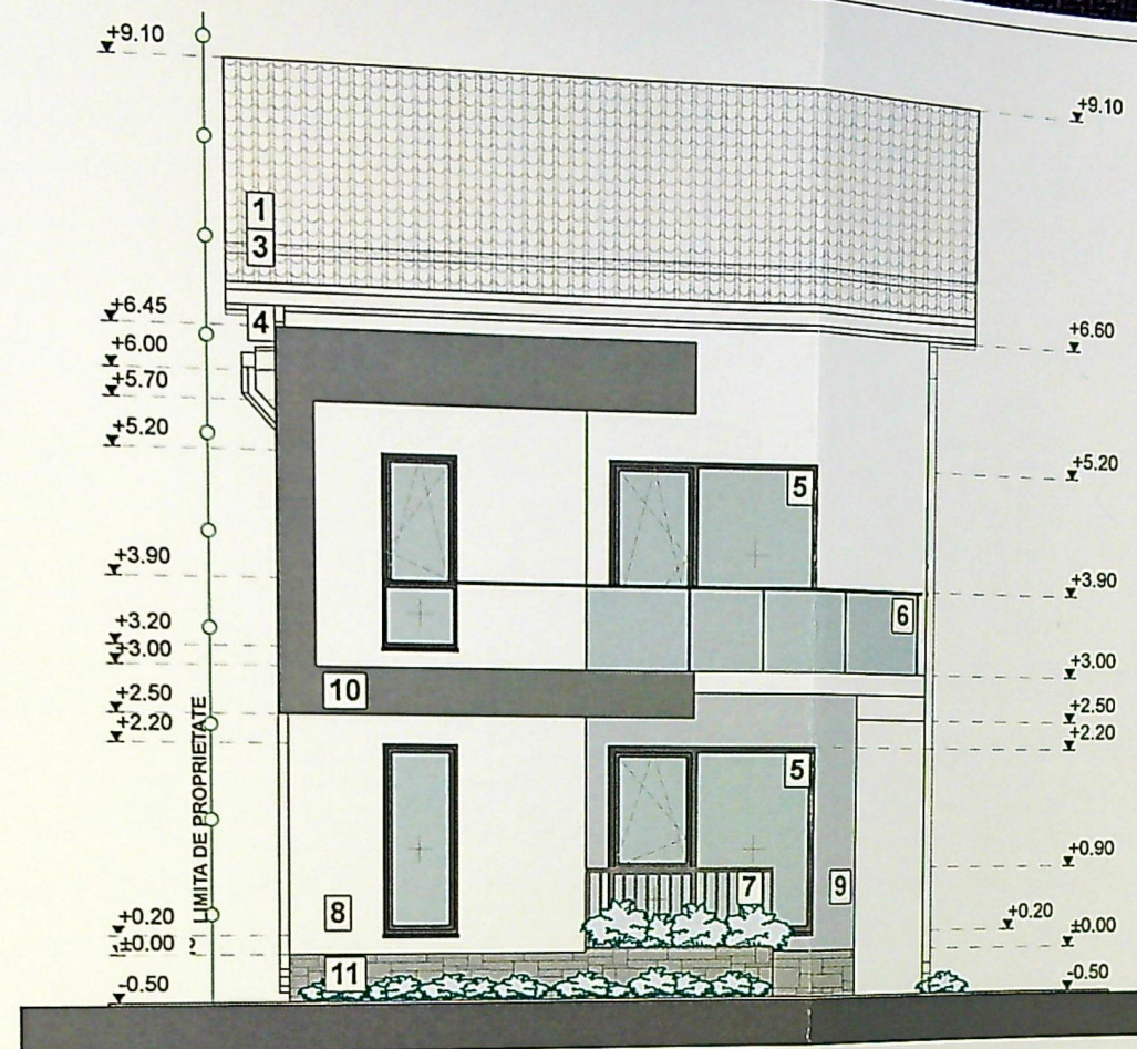
FATADA PRINCIPALA (FRONT STRADAL)
