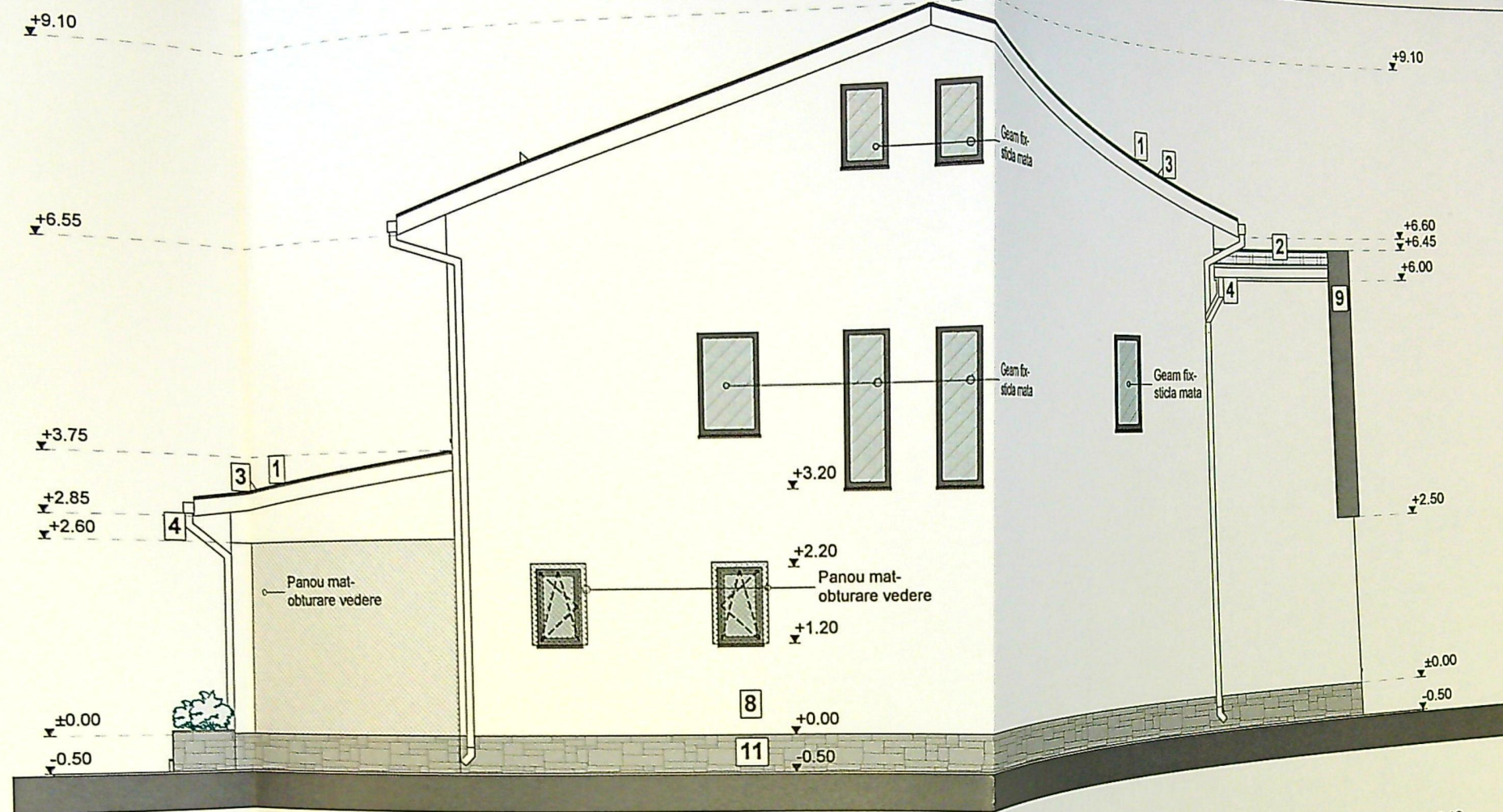
FATADA LATERALA STANGA
