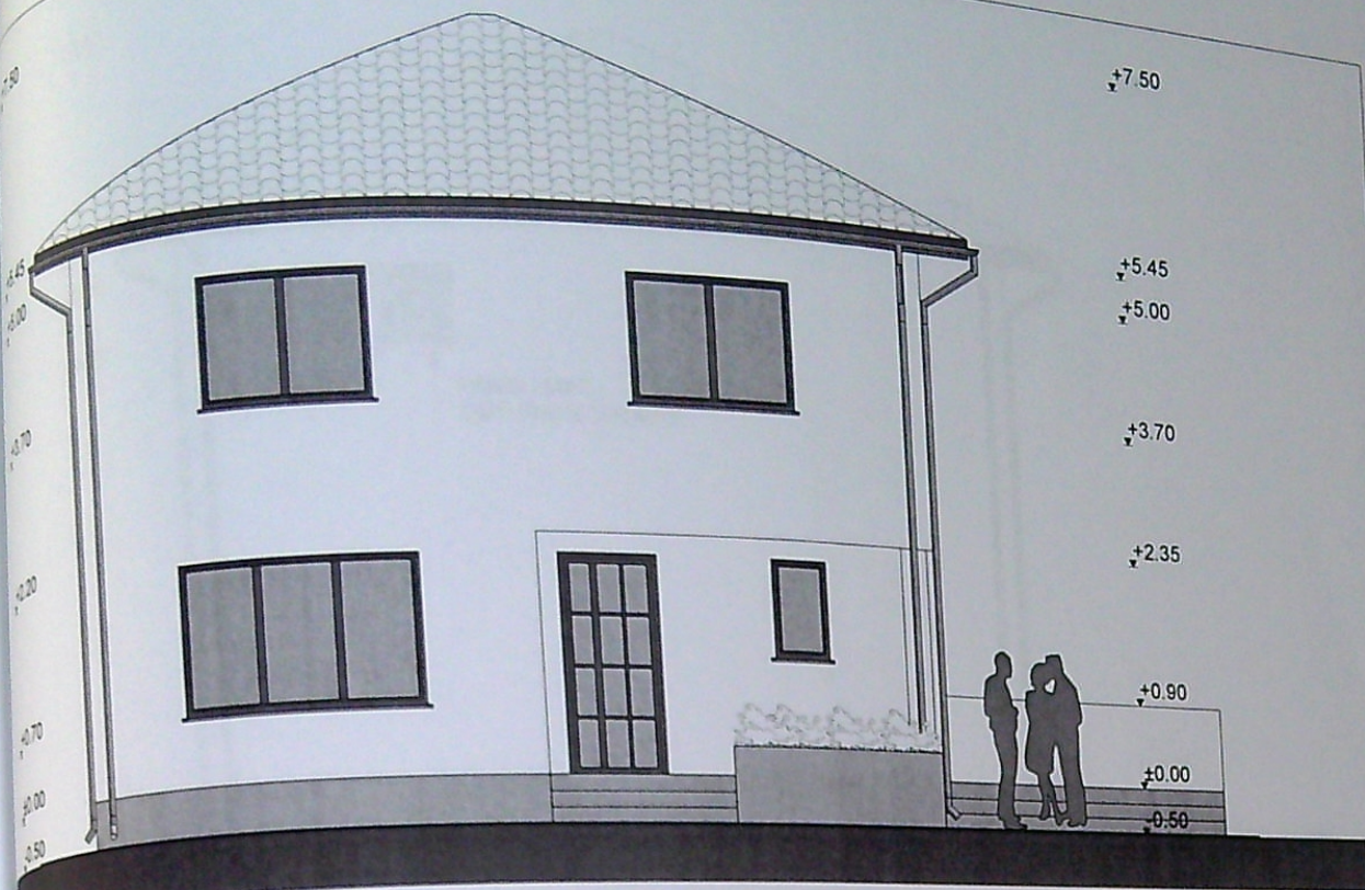
FATADA PRINCIPALA
