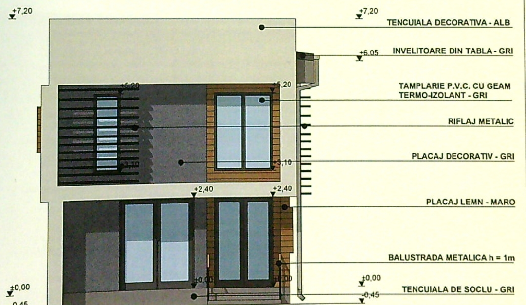
FATADA VEST
