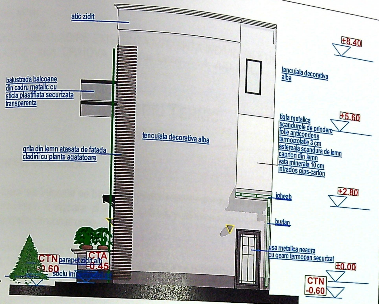
FATADA LATERALA STANGA
