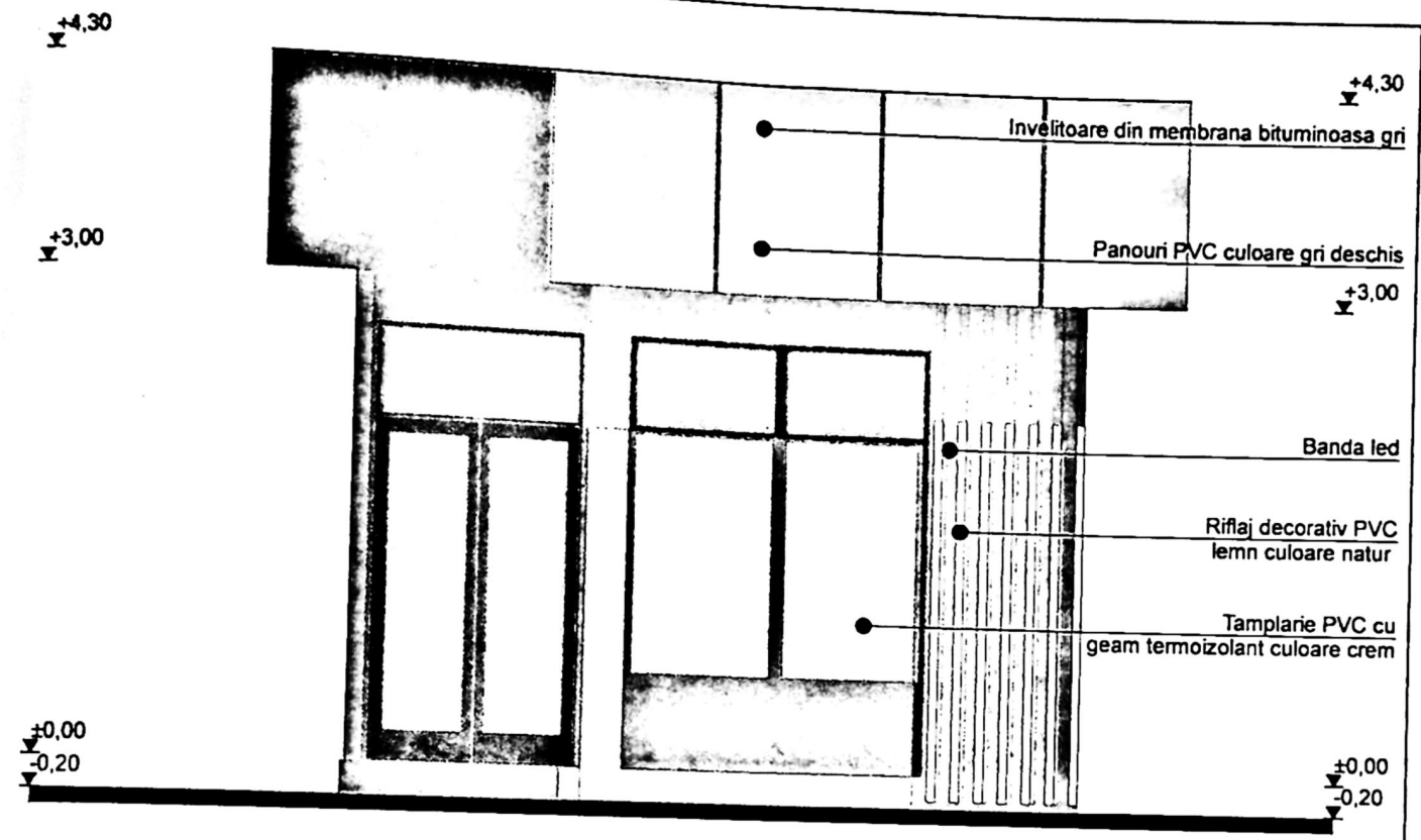
FATADA VEST
