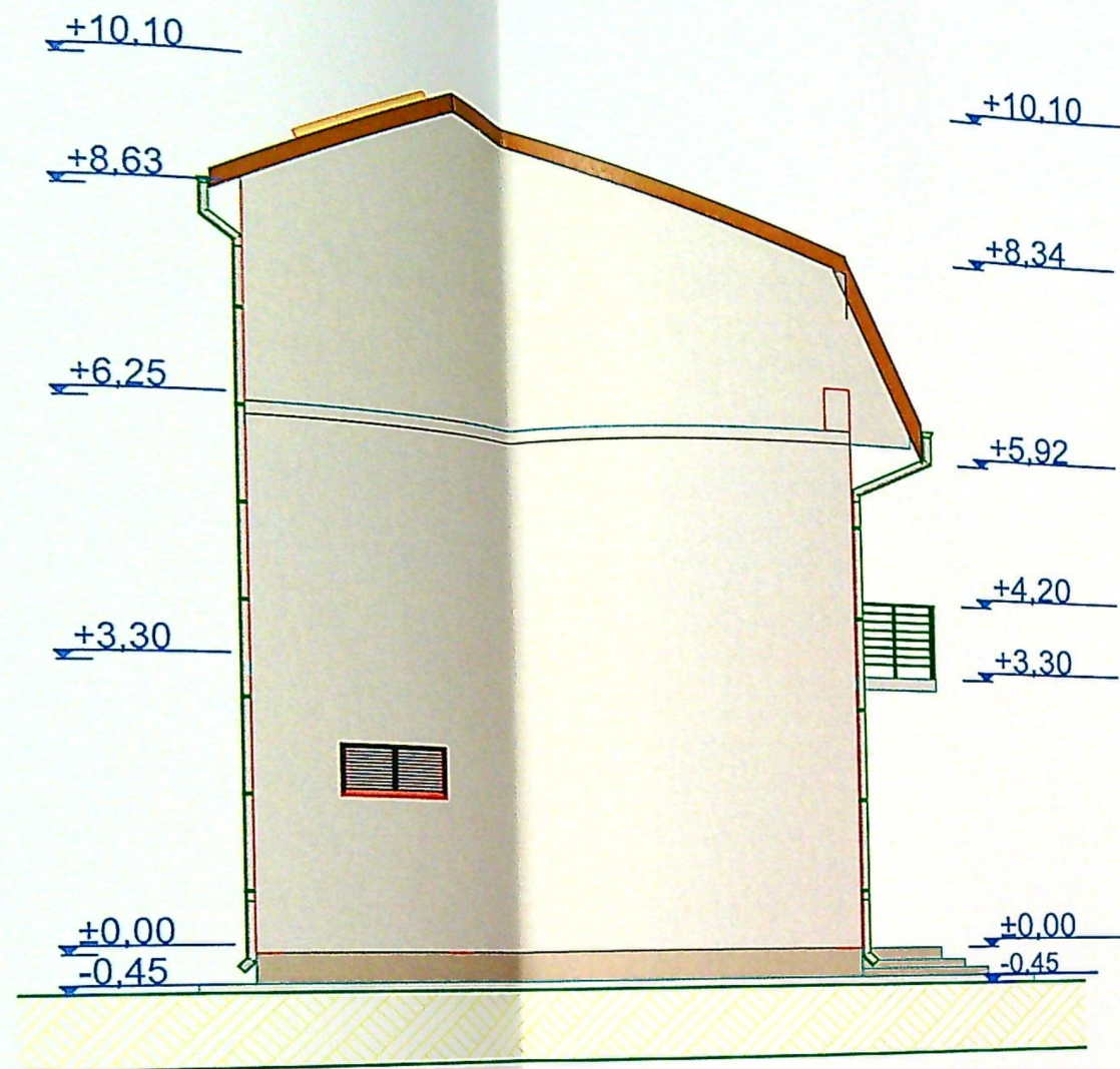
FATADA STANGA scara 1:100
