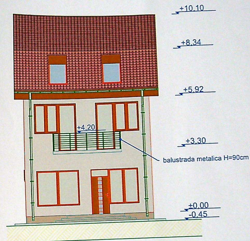
FATADA PRINCIPALA scara 1:100
